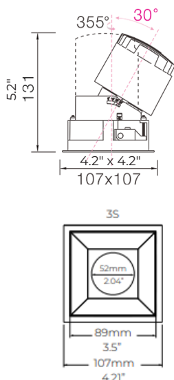
Adjustable Square
