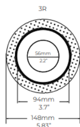
Adjustable, fixed Round
