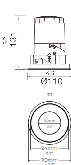
Fixed Round
