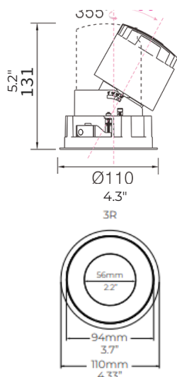
Adjustable Round
